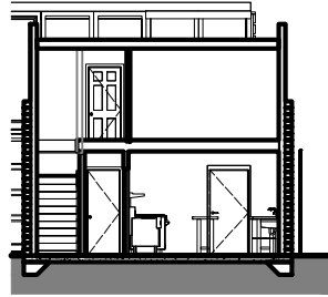
Section 4 1/4" = 1'-0"
