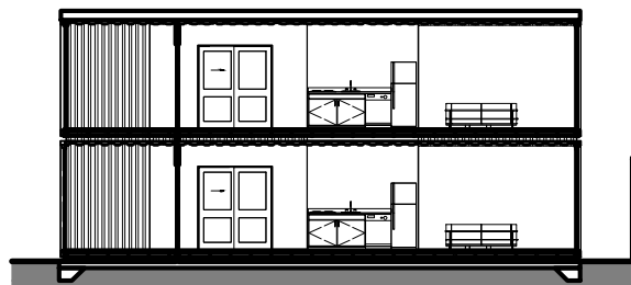
Section 3 1/4" = 1'-0"
