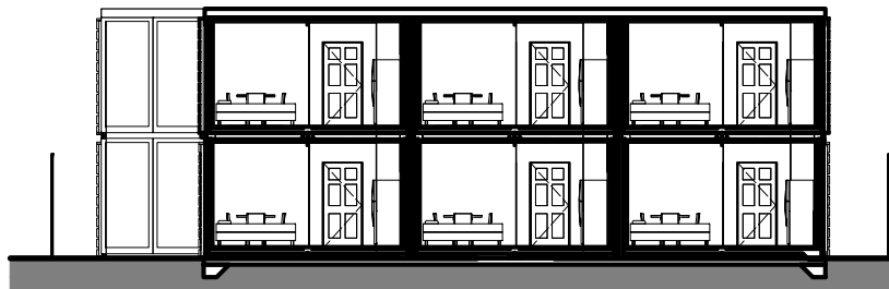
Section 1 1/4" = 1'-0"
